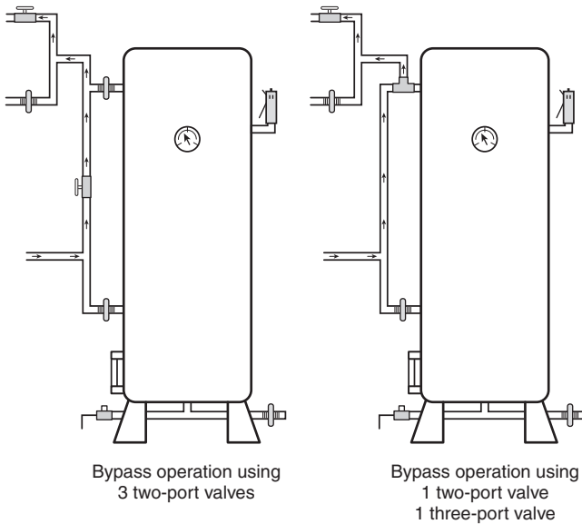
FIGURE A.5.1.3.6.3.10(D) Receiver Valving Arrangement.
