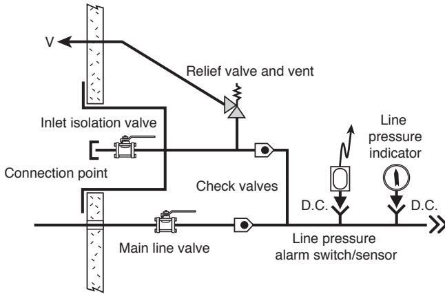
FIGURE A.5.1.3.5.13 Emergency Oxygen Supply Connection.
