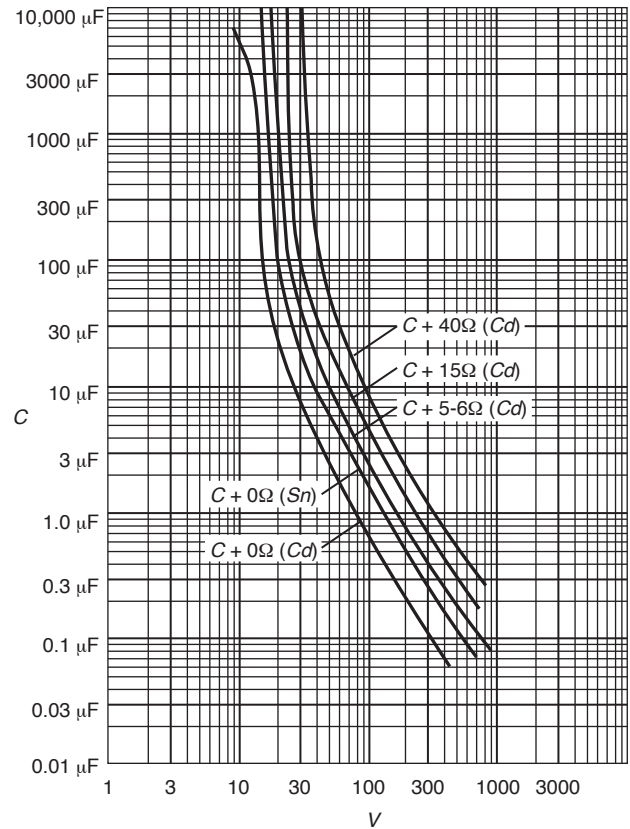
FIGURE 10.5.4.1(f) Capacitance Circuits Minimum Ignition Voltages. (The curves correspond to values of current-limiting resistance as indicated. The curve marked Sn is applicable only where cadmium, zinc, or magnesium can be excluded.)
