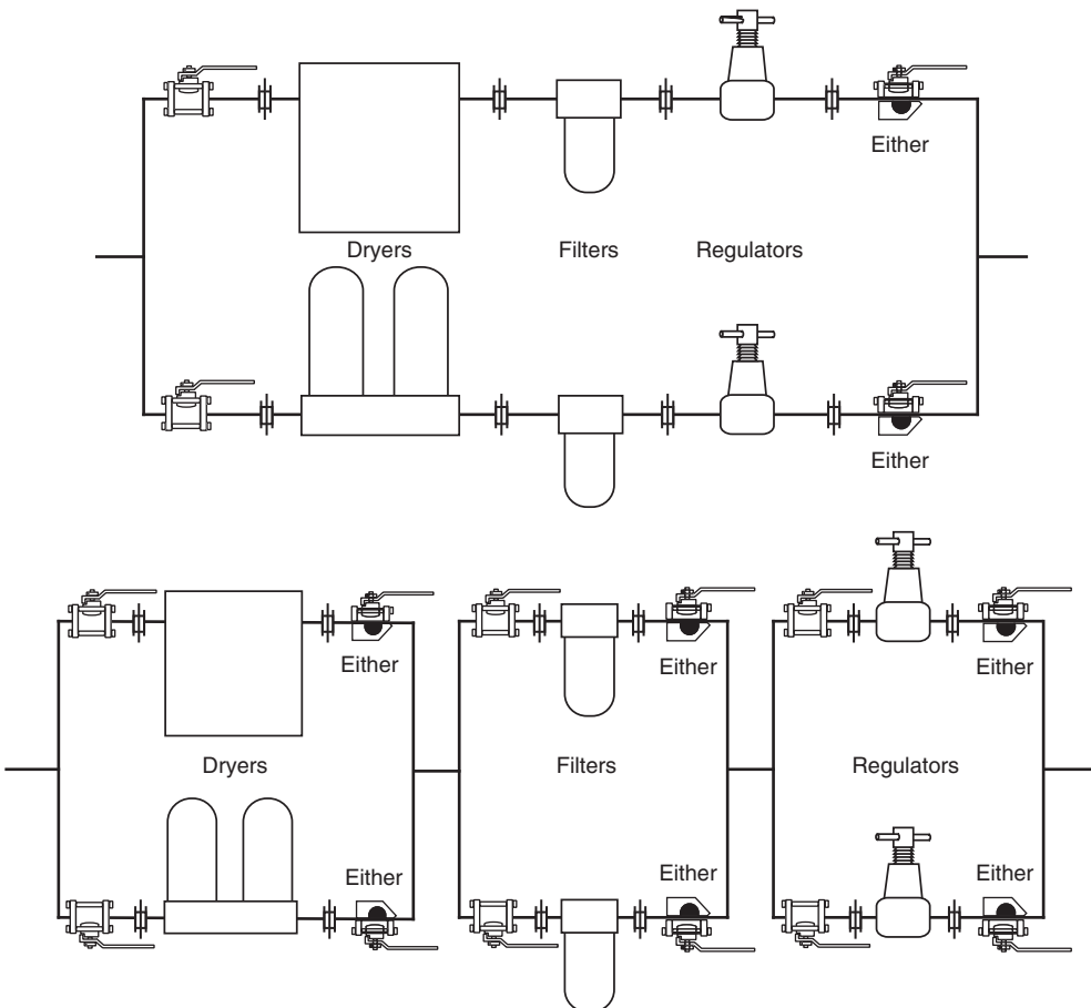
FIGURE A.5.1.3.6.3.10(F) Alternate Valving Sequences for Line Controls in Medical Air.
